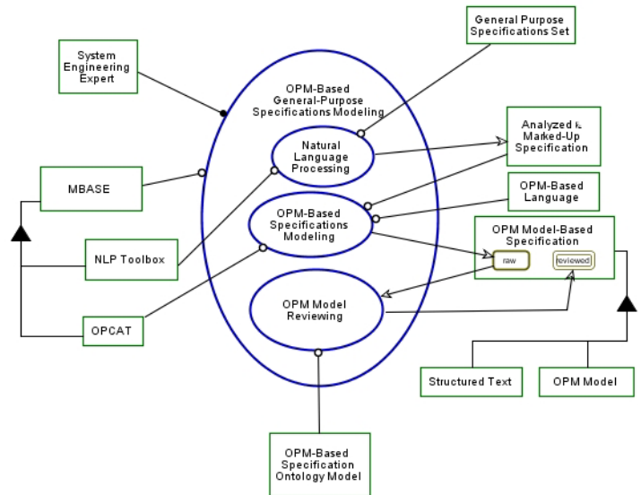
Fig. 4: Refined (second-level) OPD of the OPM-Based General Purpose Specifications zoomed in, showing the details of the process.
