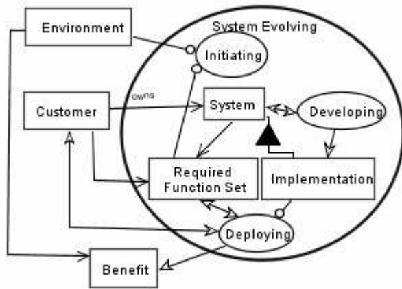
Figure 2: In zoomed OPM model of the System Evolving process
