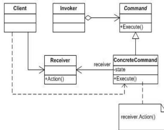
Figure 3. An OPM model of the Command design pattern [2]
