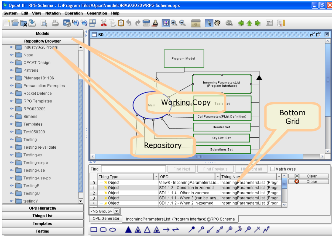
Figure 1. The Working Copy, Repository, and Bottom Grid
